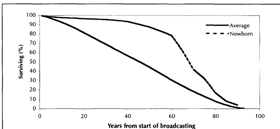
Fig. 1. Survival function for the average population (solid line) and for newborn babies (dashed line).
